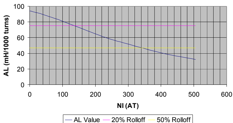
Typical AL Values Core: 0077935A7
