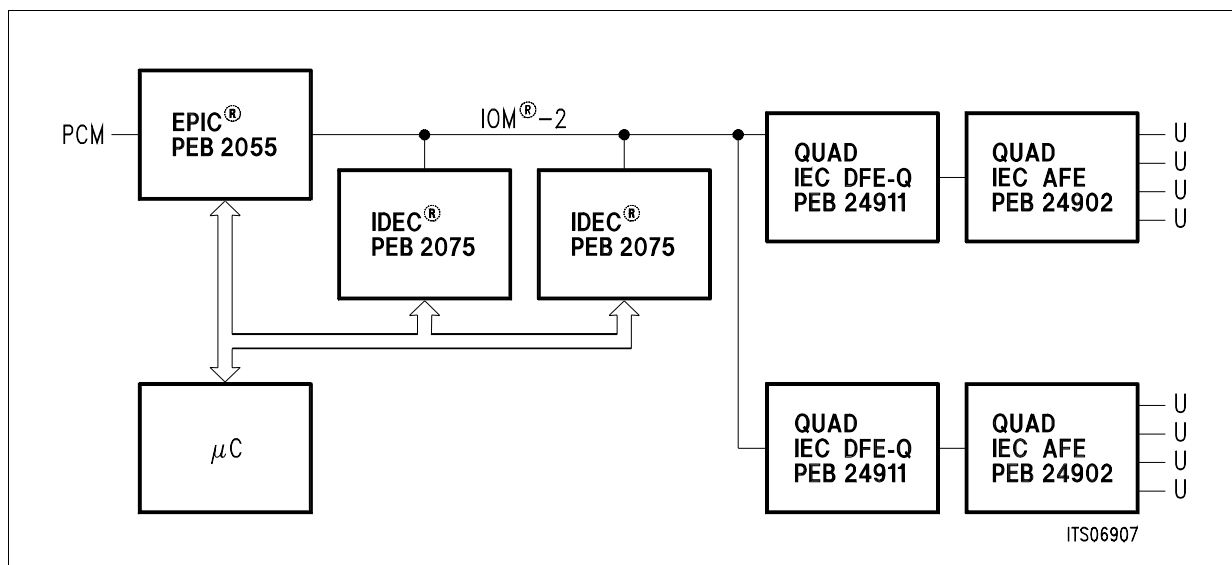
Figure 5 8 channel LT application (overview)
