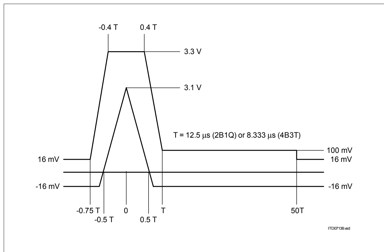
Figure 11 Pulse Mask for a Single +3 Pulse (not to scale)
