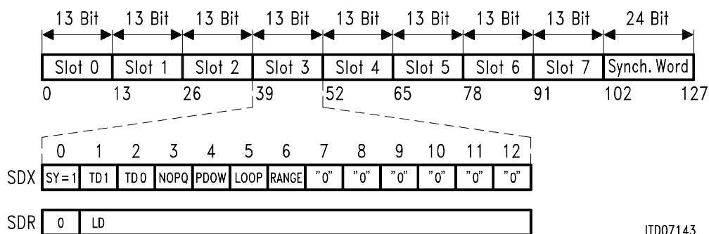
Figure 18 Frame Structure on SDX/SDR in 4B3T Mode
