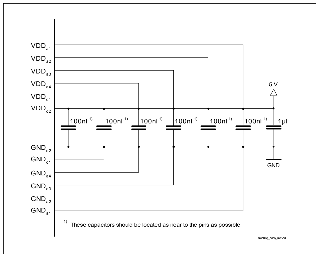
Figure 21 Power Supply Blocking
