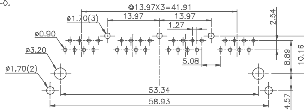
PC Board Layout Component Side Shown
