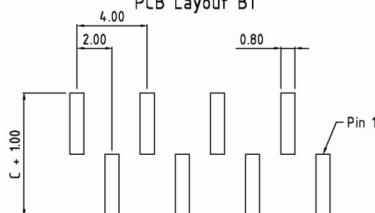
PCB Layout B1
