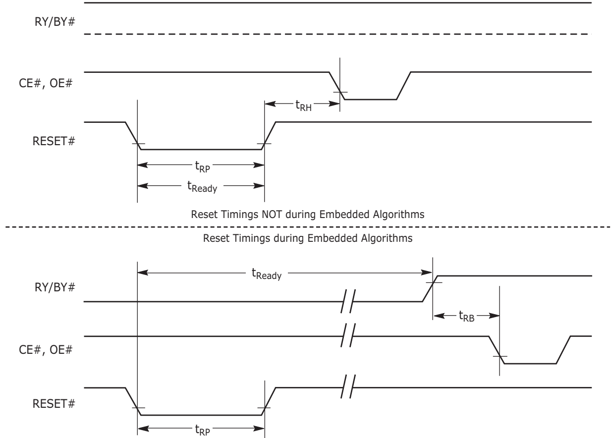
Figure 15. Reset Timings
