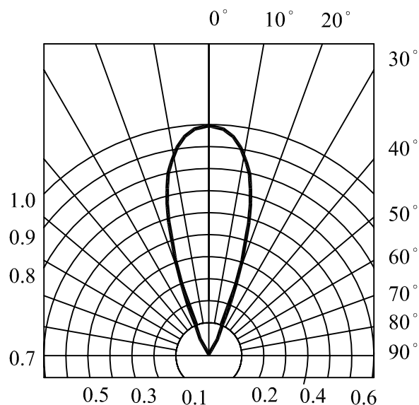
RADIATION DIAGRAM
