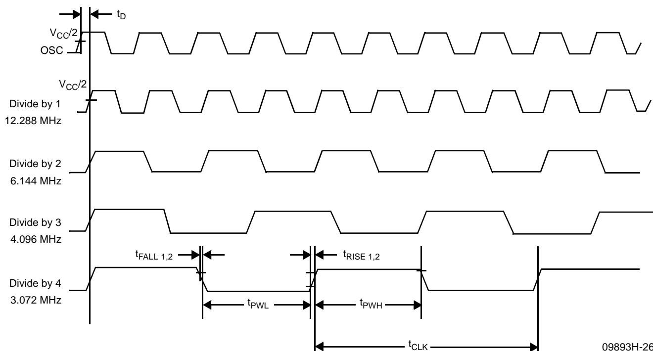
Figure 34. OSC/MCLK Timing
