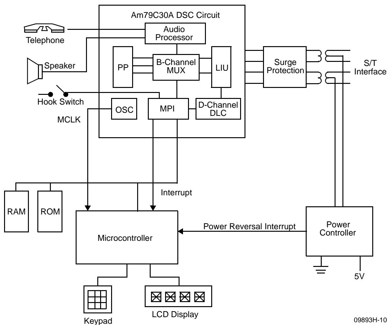
Figure 14. ISDN Telephone
