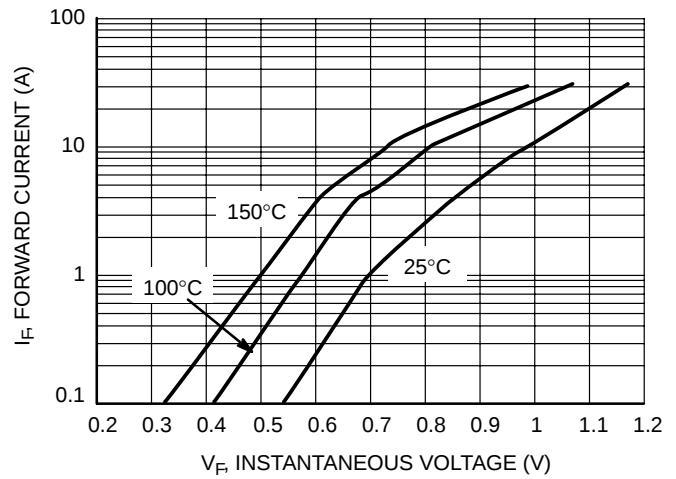
Figure 2. Maximum Forward Value Voltage
