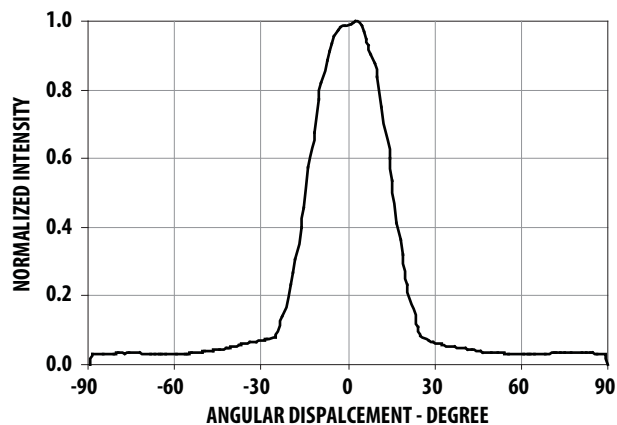
Figure 8. Radiation Pattern for 30°
