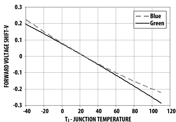
Figure 10. Relative Forward Voltage vs Junction Temperature
