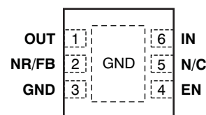
DRV PACKAGE 2mm × 2mm SON-6 (TOP VIEW)
