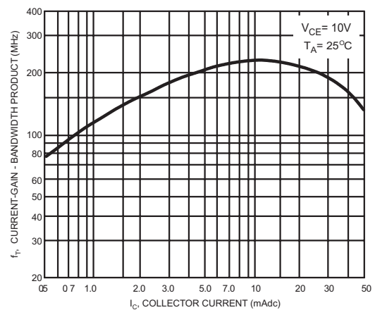
FIG.6- CURRENT-GAIN - BANDWIDTH PRODUCT
