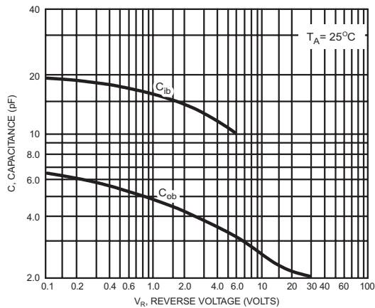
FIG.11- CAPACITANCES
