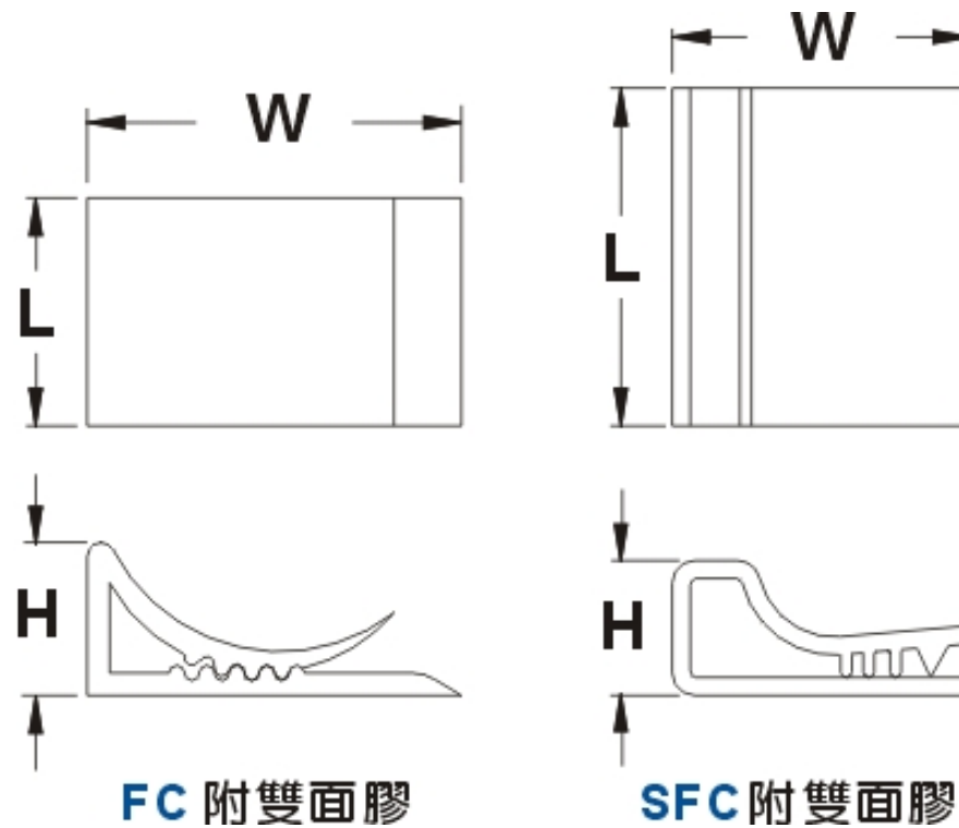
ADHESIVE TAPE
