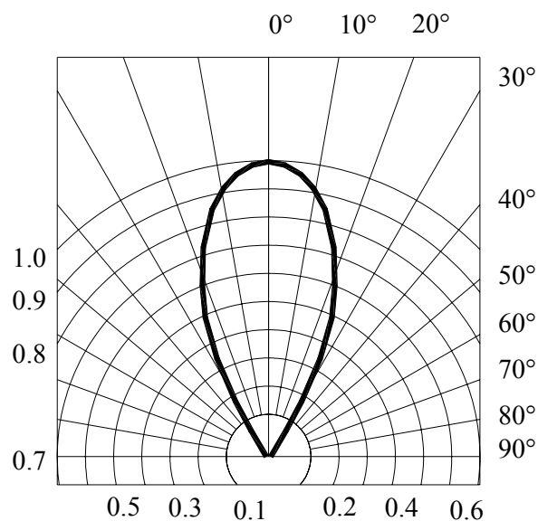
RADIATION DIAGRAM
