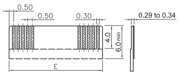
APPLICABLE FFC LAYOUT
