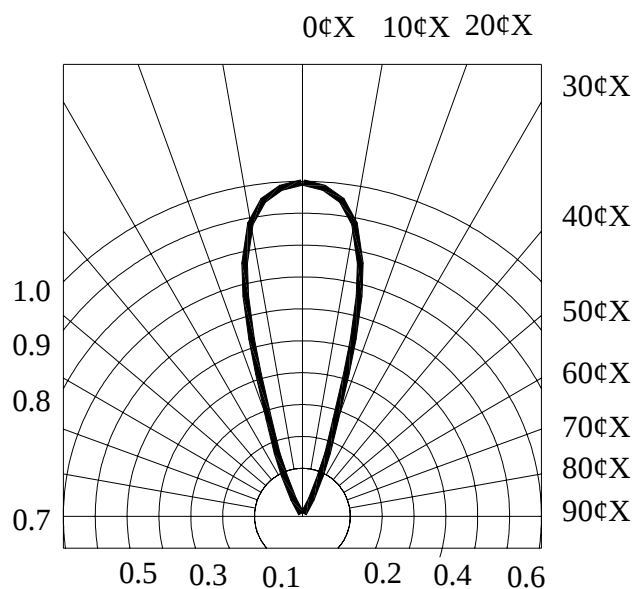
RADIATION DIAGRAM
