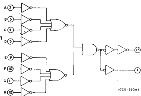
Fig. 1 — Logic diagram.
