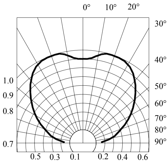
RADIATION DIAGRAM
