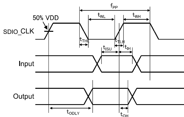
SDIO Bus Timing (a) parameters (High-Speed Mode)
