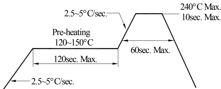
< 1 : Lead Solder >
