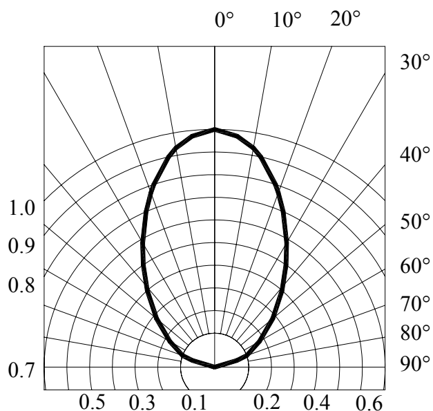
RADIATION DIAGRAM
