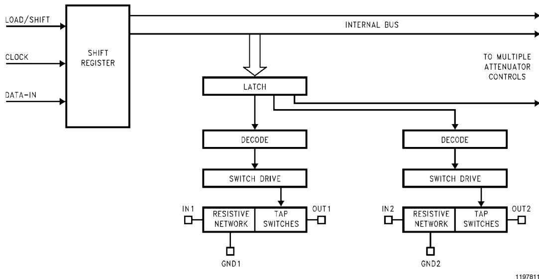
FIGURE 9. μPot System Architecture
