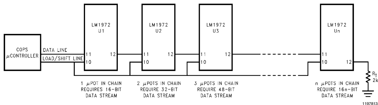
FIGURE 11. n- \mu Pot Daisy-Chained Circuit
