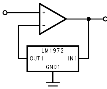
FIGURE 10. Digitally-Controlled Logarithmic Gain Amplifier Circuit
