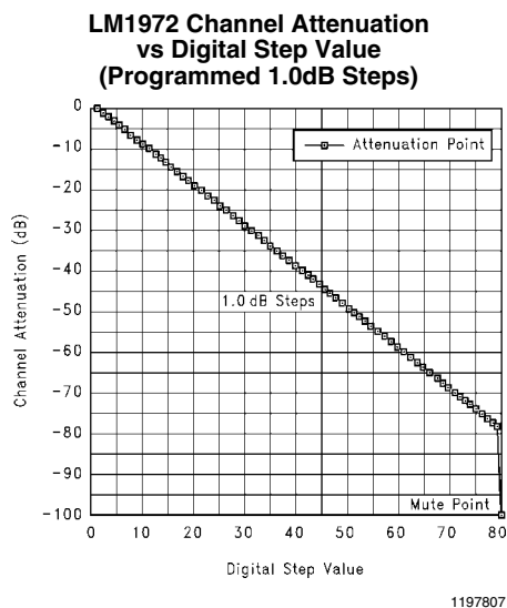
FIGURE 4. LM1972 1.0dB Attenuation Step Scheme
