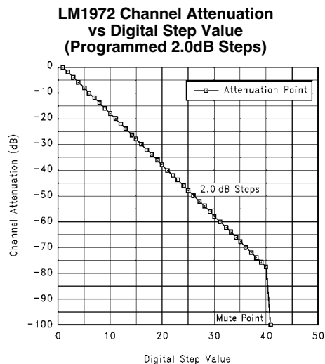
FIGURE 5. LM1972 2.0dB Attenuation Step Scheme
