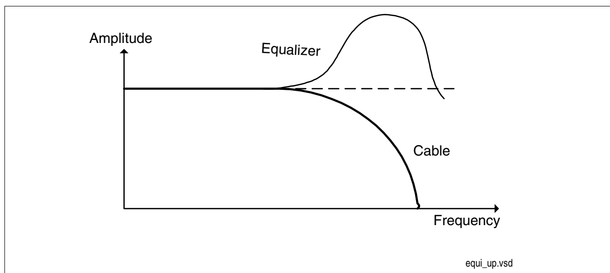
Figure 12 Equalizer Effect
