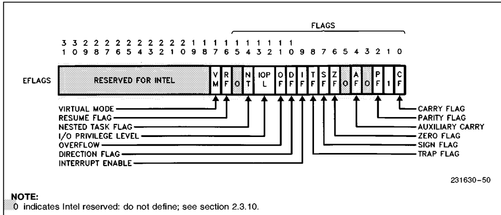
Figure 2-3. Flags Register
