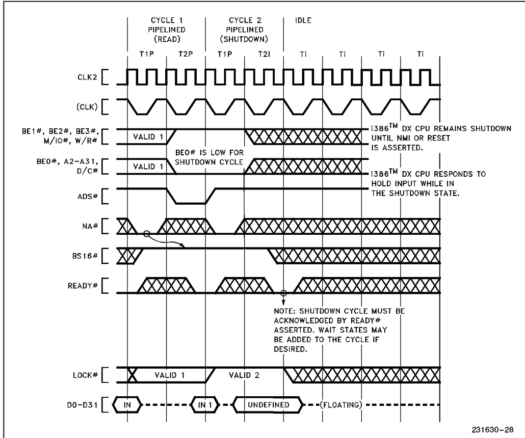
Figure 5-24. Shutdown Indication Cycle
