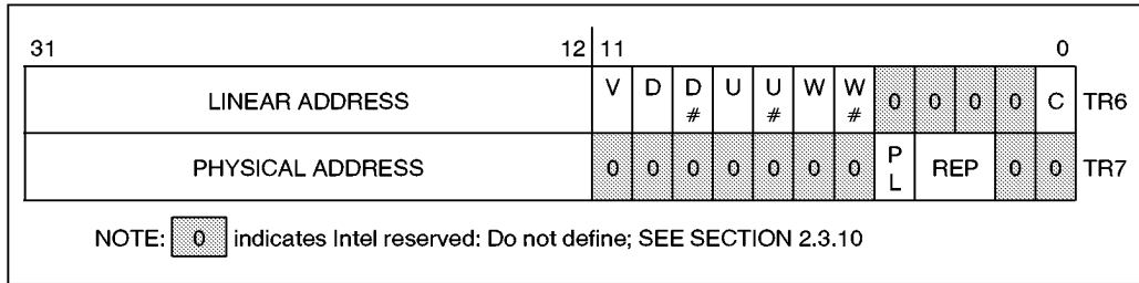
Figure 2-12. Test Registers
