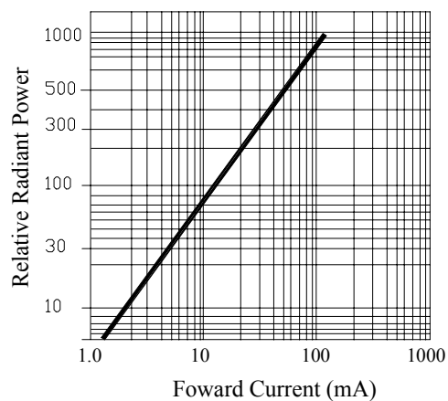
FORWARD CURRENT VS. LUMINOUS INTENSITY
