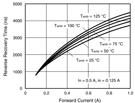
Figure 6. Reverse Recovery Time vs. Forward Current
