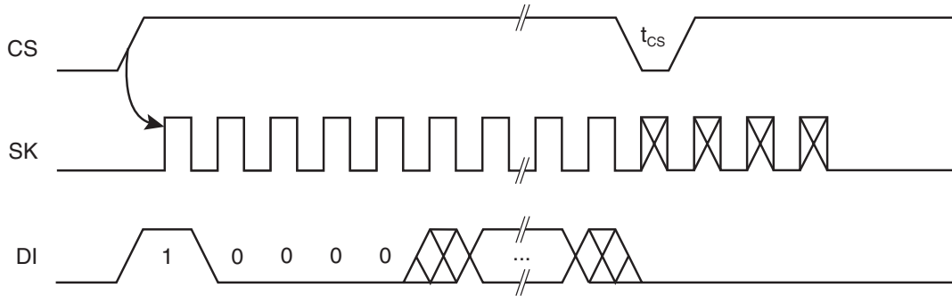
Figure 5. EWDS Timing
