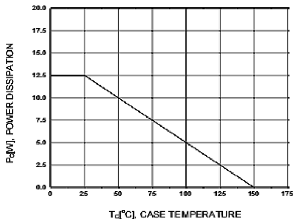
Fig 3: Power Derating
