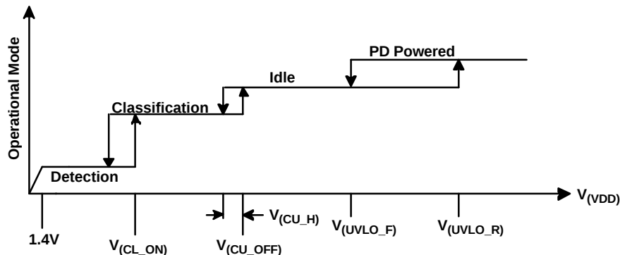
Figure 17. Threshold Voltages
