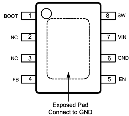
8-Lead Plastic PSOP-8 Package NS Package Number MRA08B
