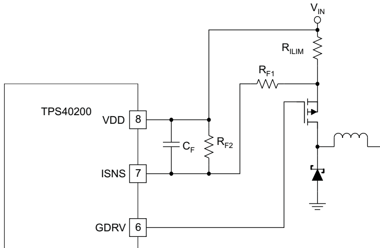
Figure 30. Current Limit Adjustment
