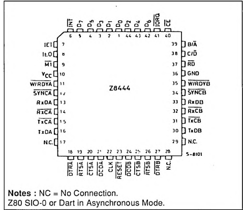
Figure 7 : Chip Carrier Pin Configuration.
