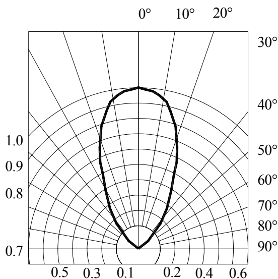
RADIATION DIAGRAM
