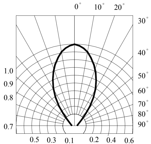
RADIATION DIAGRAM
