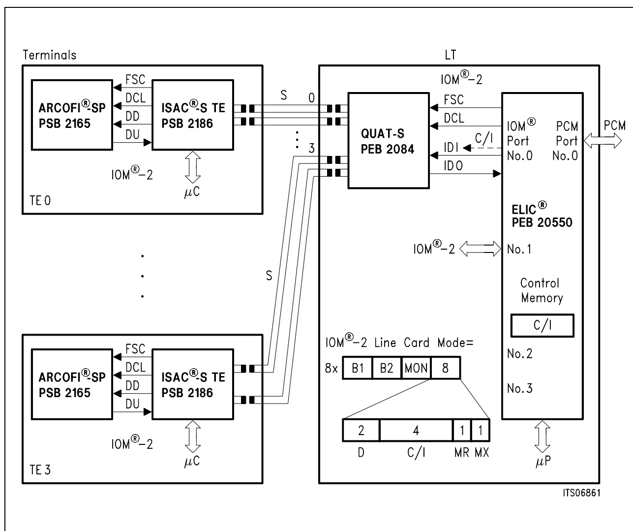
Figure 6 System Integration, IOM ® -2 Interface
