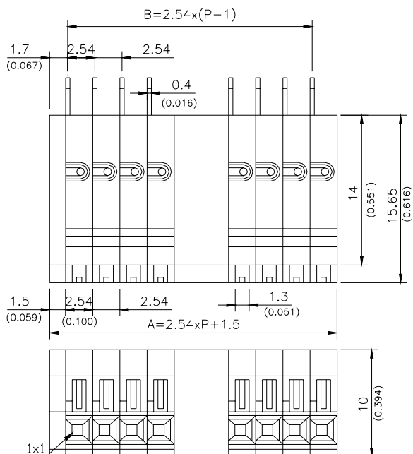
ETB64 Drawing DIMENSIONS UNIT:mm(inch)
