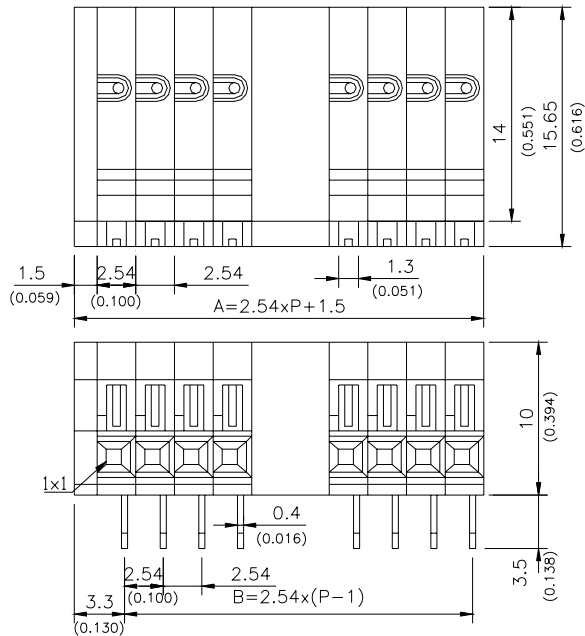
ETB63 Drawing DIMENSIONS UNIT:mm(inch)
