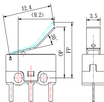
Stainless steel lever t=0.3
