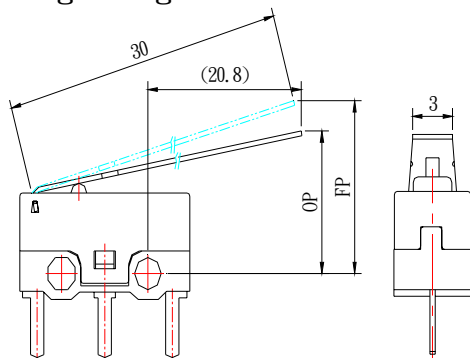
Stainless steel lever t=0.3
