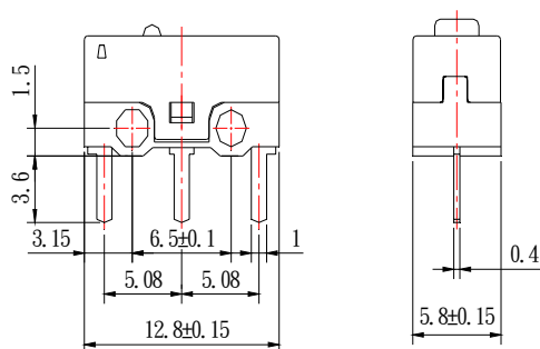
Straight Type
