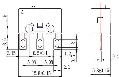
Solder Type
