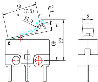
Stainless steel lever t=0.3
