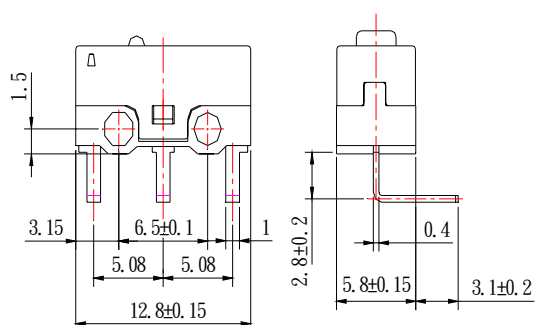
Right Type
