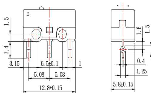
Self-Standing Type
