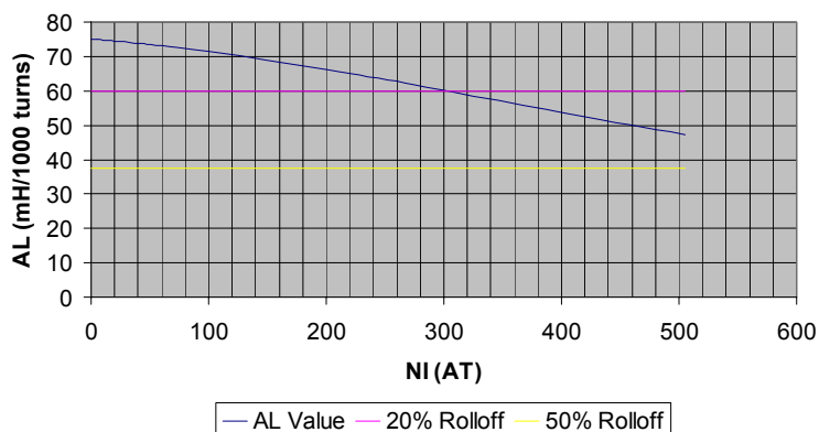
Typical AL Values Core: C058894A2
