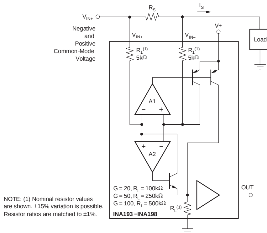
Figure 6. INA193-INA198 Simplified Circuit Diagram
