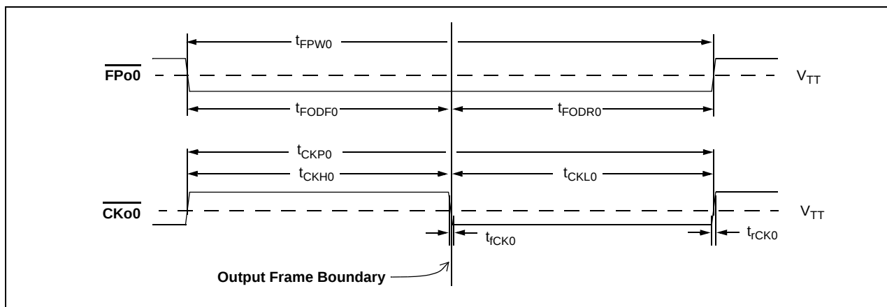
Figure 29 - \overline{\text{FPo0}} and \overline{\text{CKo0}} Timing Diagram
