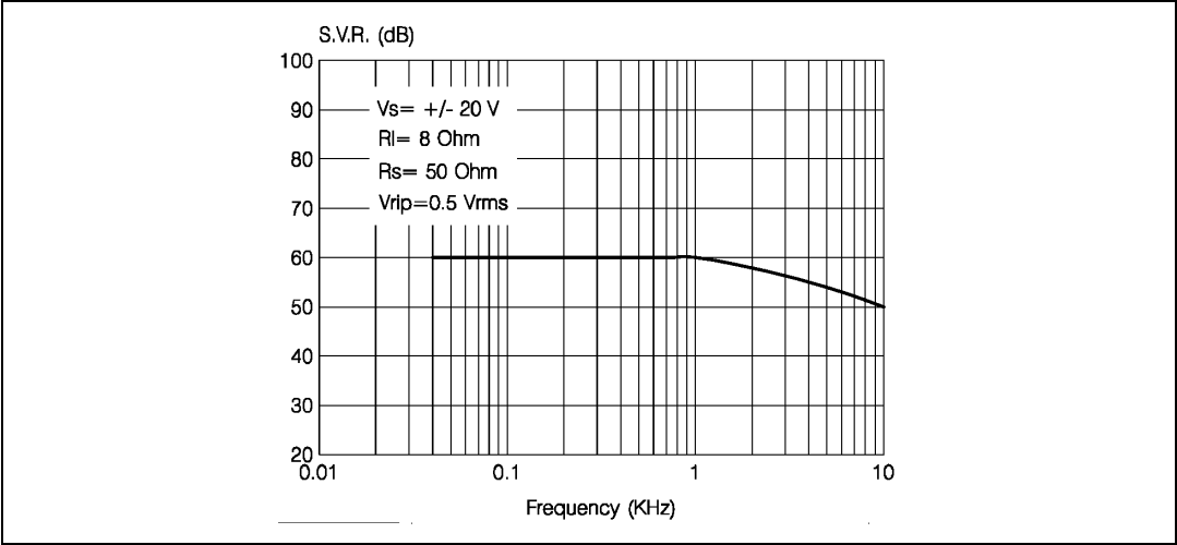
Figure 8. SVRR vs frequency
