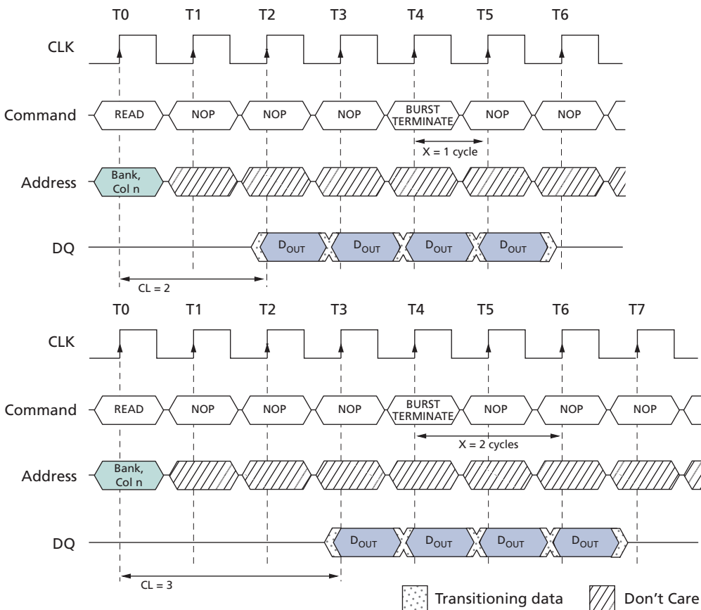
Figure 20: Terminating a READ Burst
