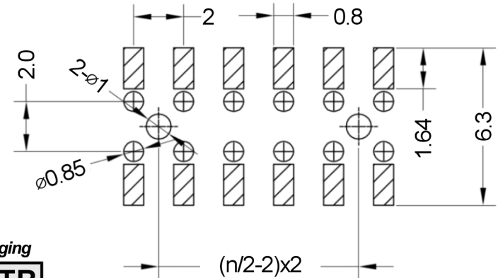
Recommended P.C.B Layout(Top Side) (PCB BOARD TOLERANCE±0.05)
