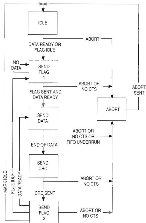
Figure 2. Transmitter State Diagram HDLC Operation
