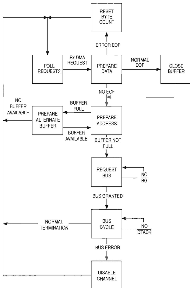
Figure 7. Receive DMA State Diagram
