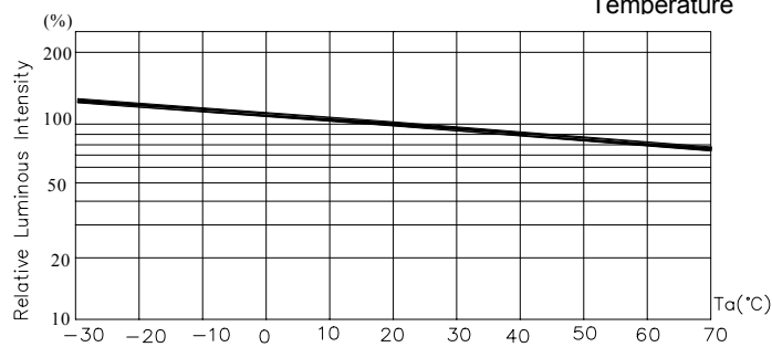
Fig.5 Luminous Intensity at I_F=70mA vs. Ambient Temperature
