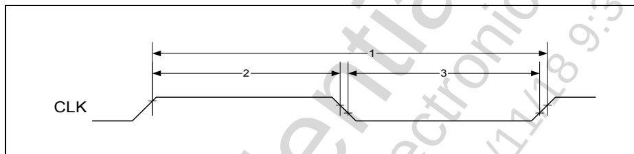
Figure 69 Microprocessor Interface Clock Timing
