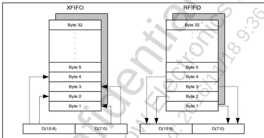
Figure 10 XFIFO/RFIFO Word Access (Intel Mode)
