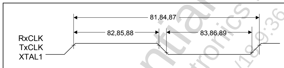
Figure 79 Clock Input Timing
