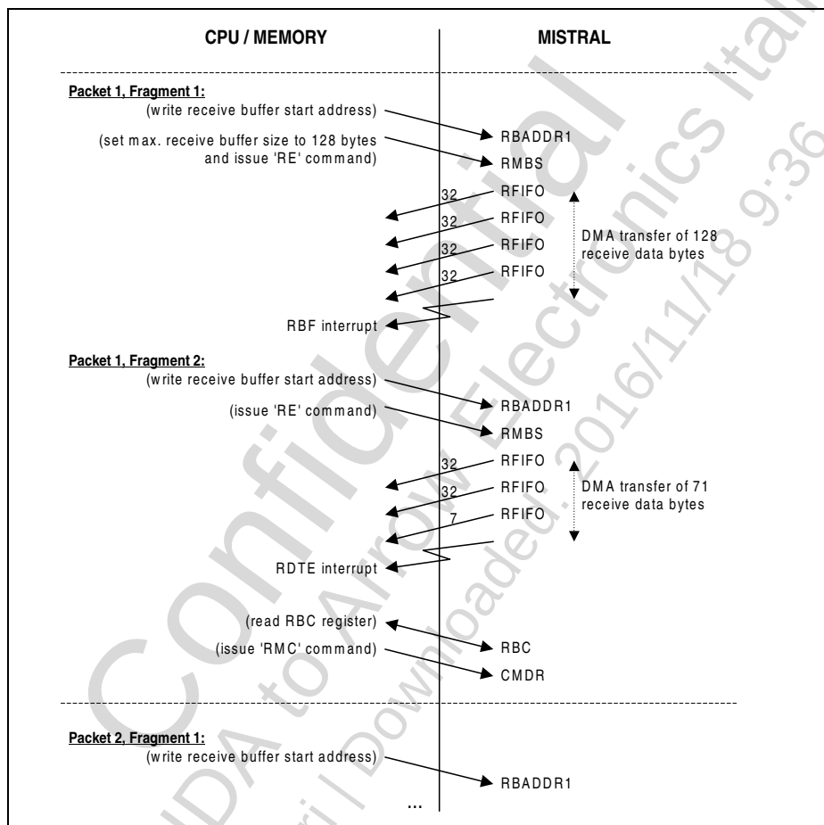
Figure 66 Fragmented Reception Sequence (Example)
