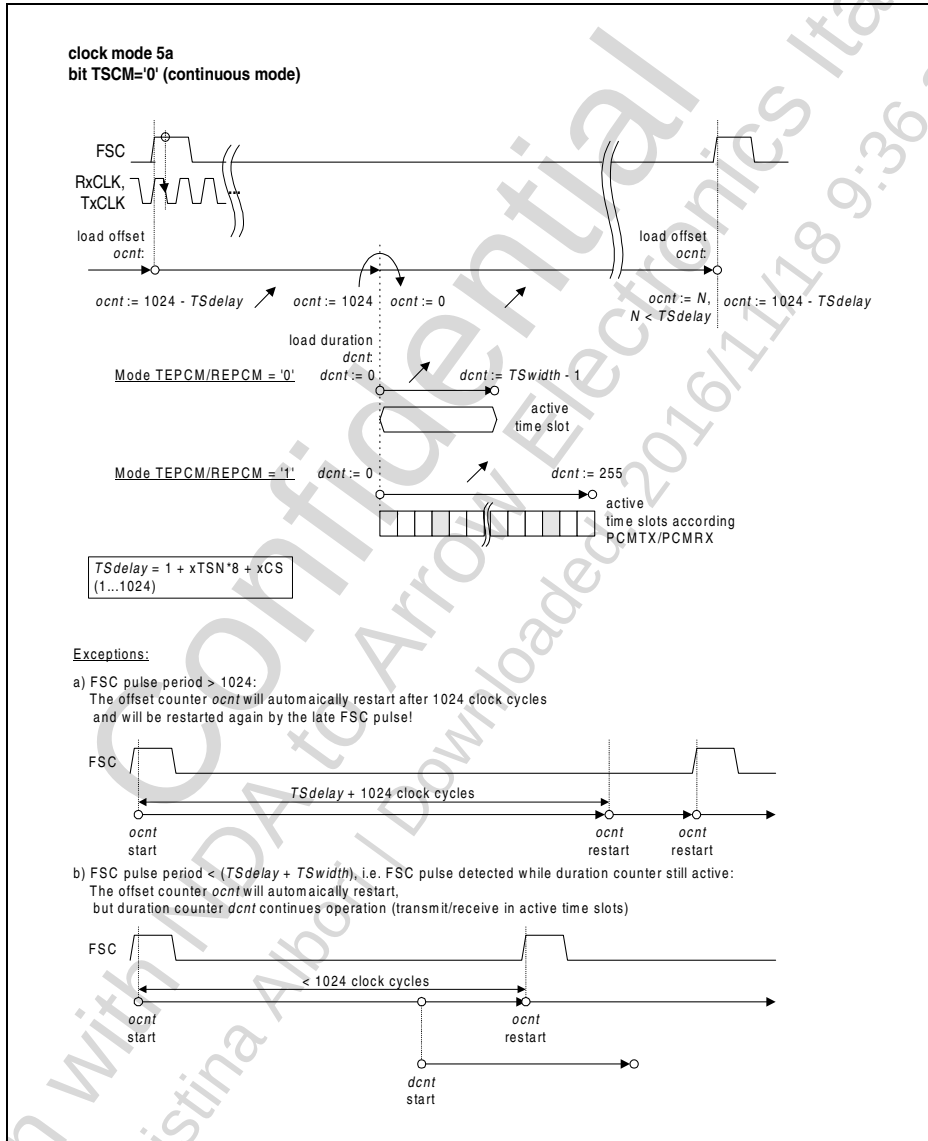
Figure 21 Clock Mode 5a "Continuous Mode"
