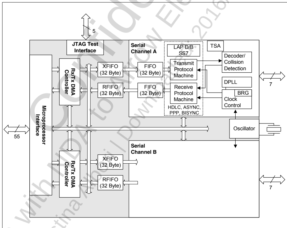
Figure 7 Block Diagram
