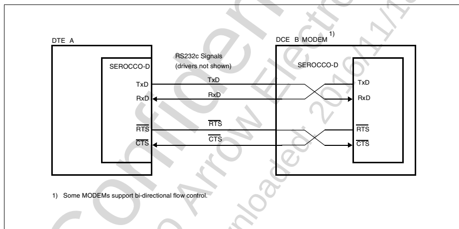
Figure 51 Out-of-Band DTE-DCE Bi-directional Flow Control
