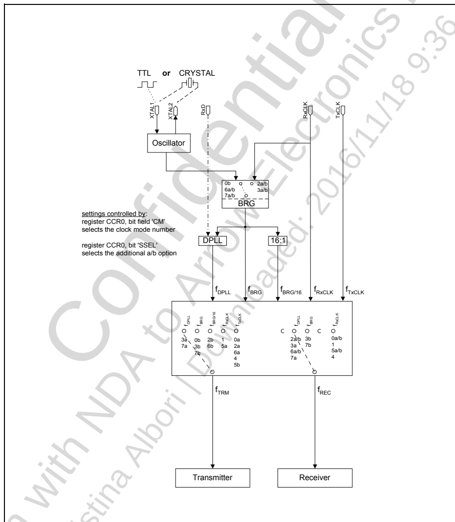
Figure 12 Clock Supply Overview
