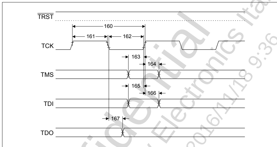
Figure 87 JTAG-Boundary Scan Timing
