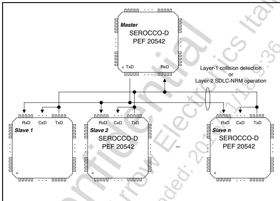
Figure 4 Point-to-Multipoint Bus Configuration
