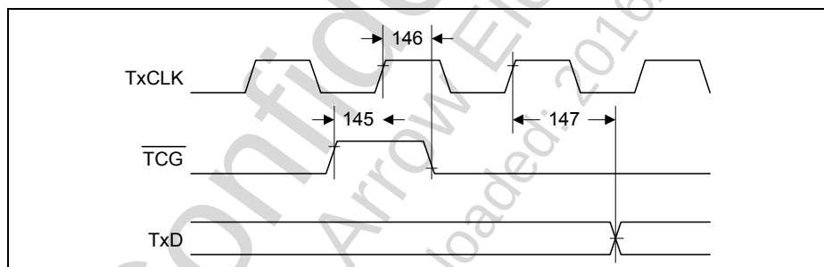
Figure 84 Clock Mode 4 Transmit Gating Timing
