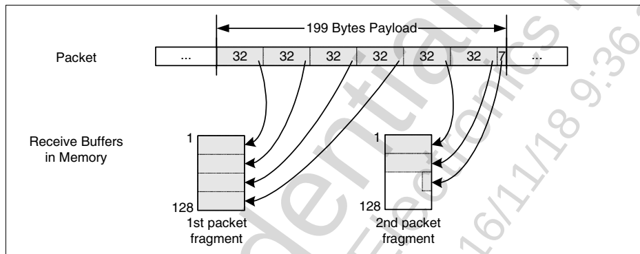
Figure 65 Fragmented Reception per DMA (Example)
