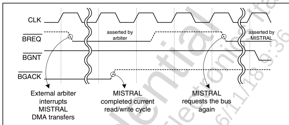
Figure 38 Bus Preemption and Re-gain of Bus Control
