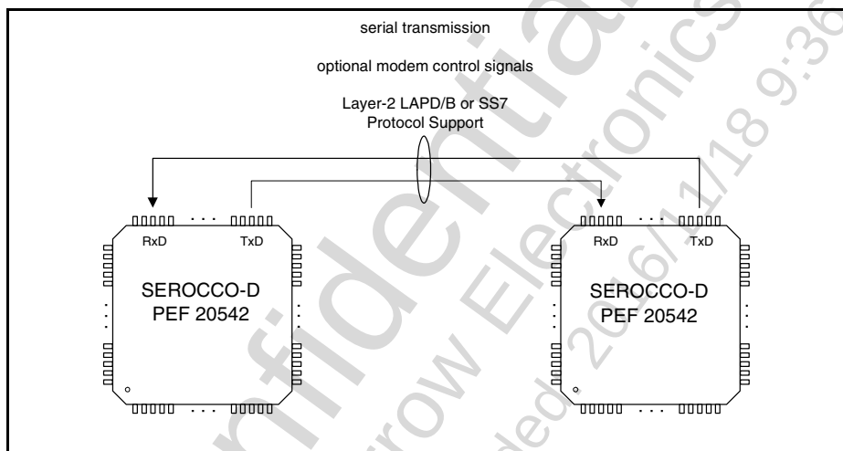
Figure 3 Point-to-Point Configuration
