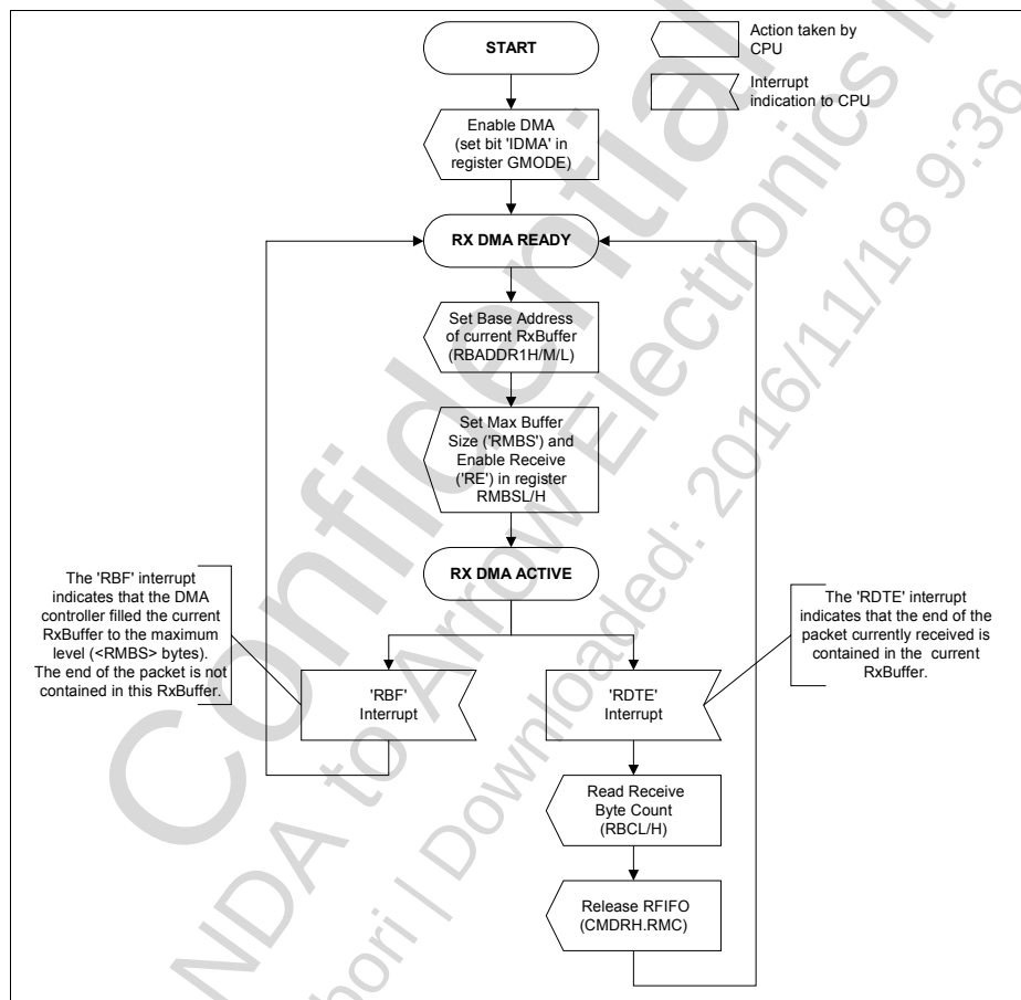
Figure 67 DMA Controlled Data Reception (Flow Diagram)
