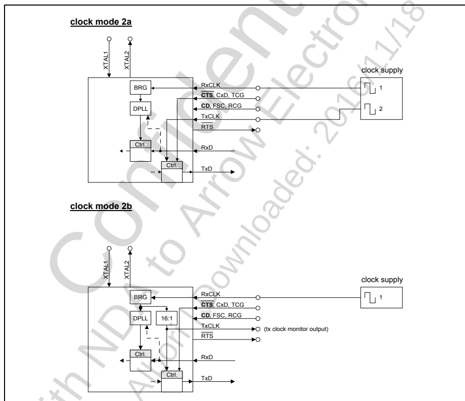
Figure 15 Clock Mode 2a/2b Configuration
