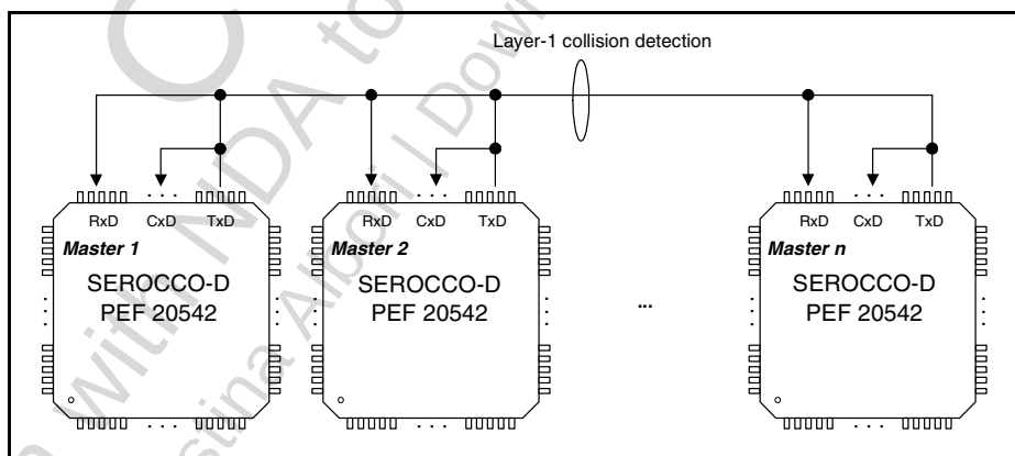
Figure 5 Multimaster Bus Configuration
