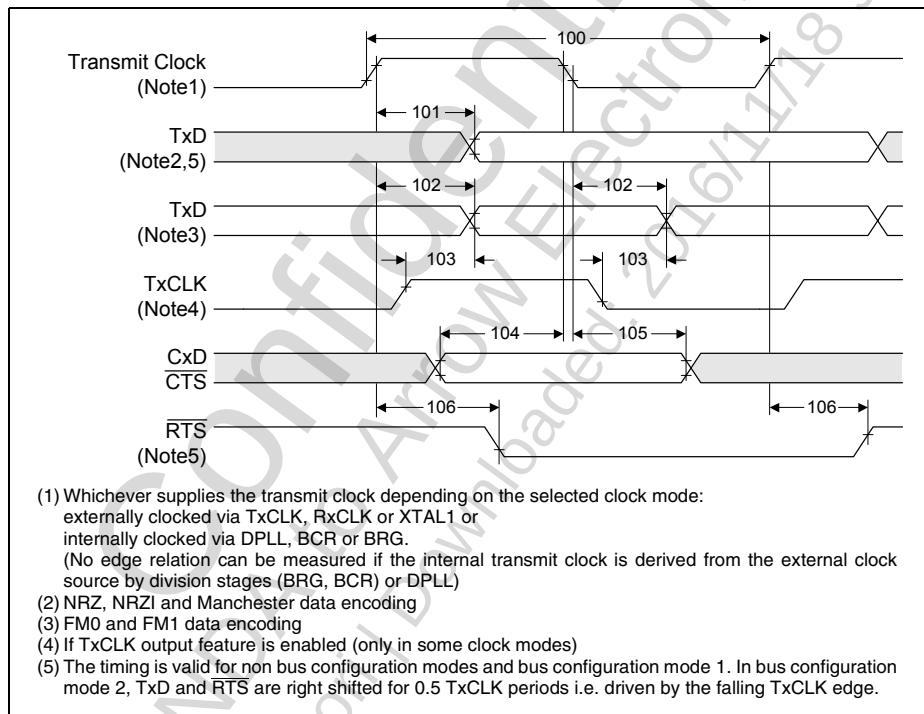
Figure 81 Transmit Cycle Timing
