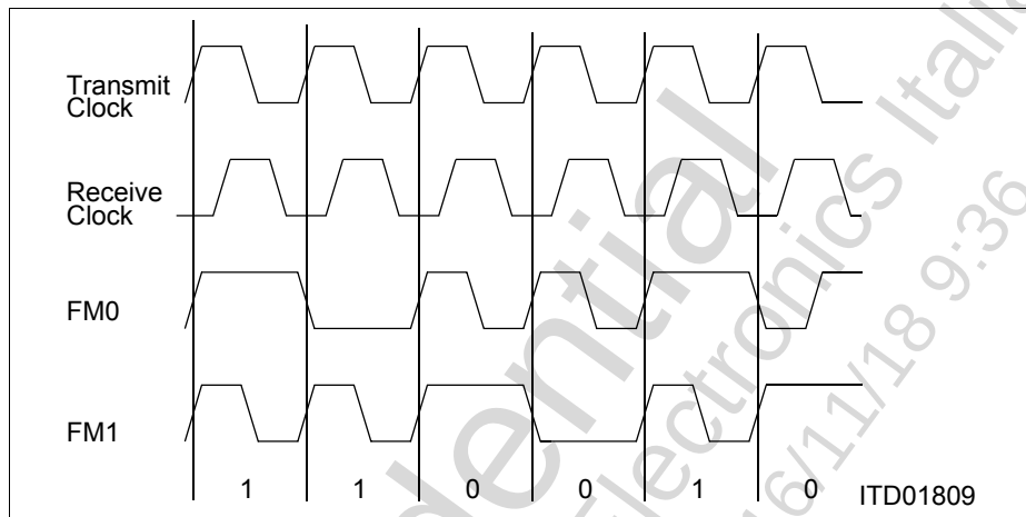
Figure 32 FM0 and FM1 Data Encoding
