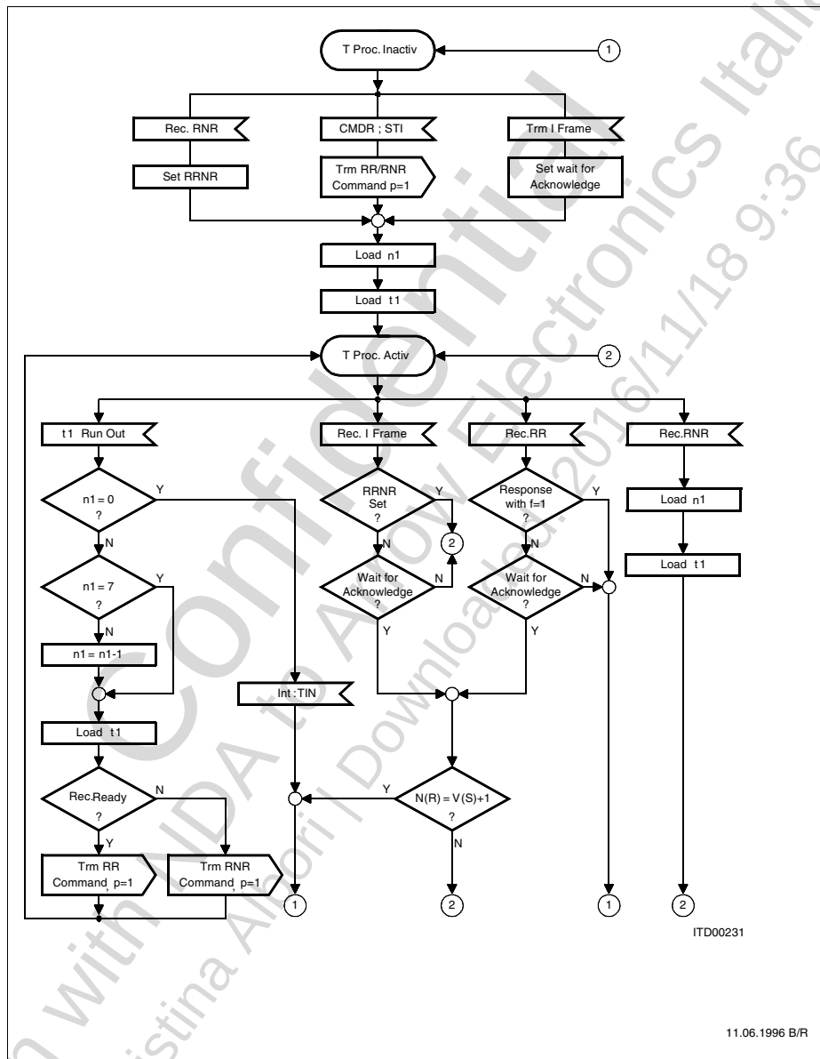
Figure 54 Timer Procedure/Poll Cycle
