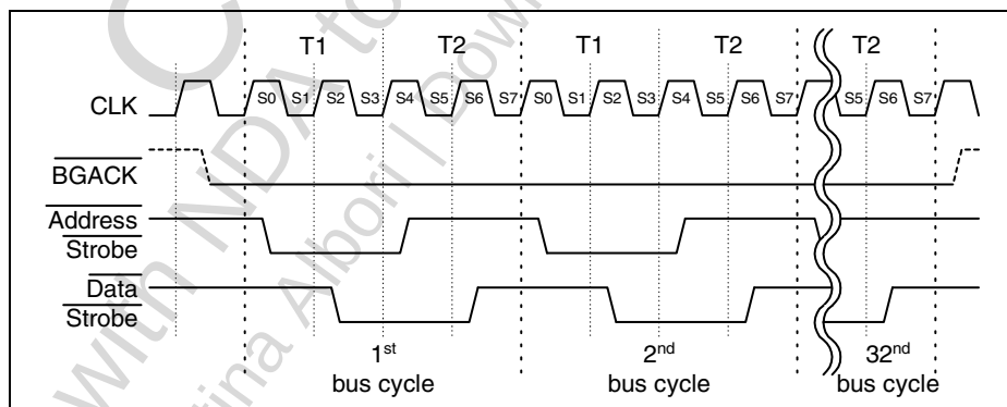
Figure 37 Un-interrupted Series of 32 DMA Bus Cycles
