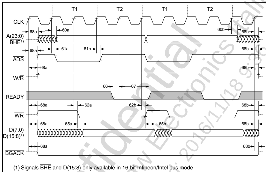
Figure 75 Infineon/Intel Write Cycle Timing (Master Access)
