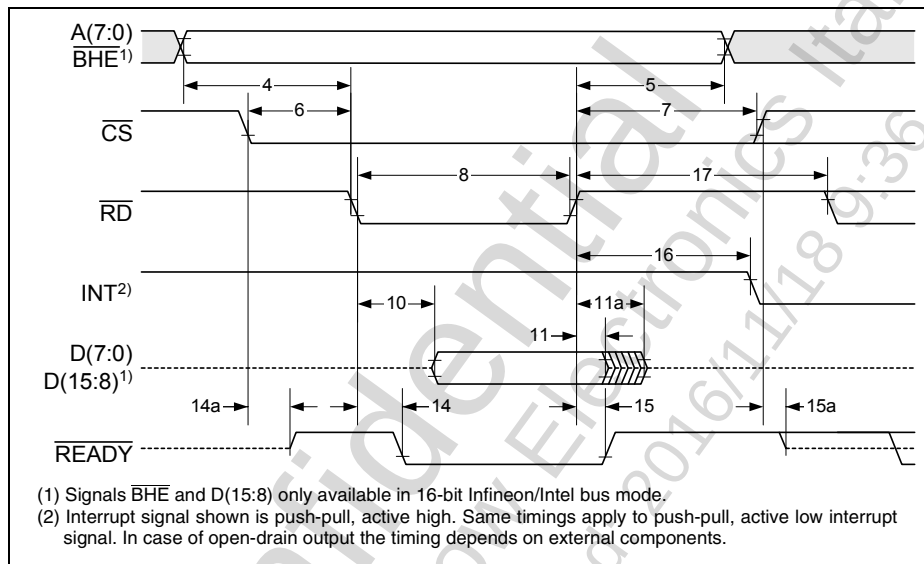
Figure 70 Infineon/Intel Read Cycle Timing (Slave Access)
