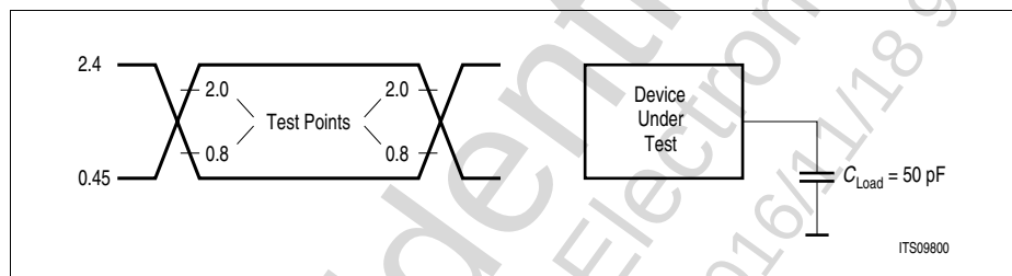
Figure 68 Input/Output Waveform for AC Tests
