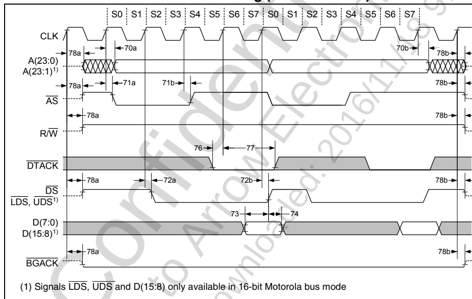
Figure 76 Motorola Read Cycle Timing (Master Access)
