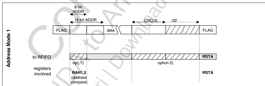
Figure 45 HDLC Receive Data Processing in Address Mode 1
