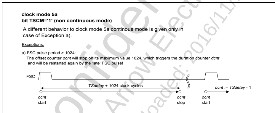
Figure 22 Clock Mode 5a "Non Continuous Mode"
