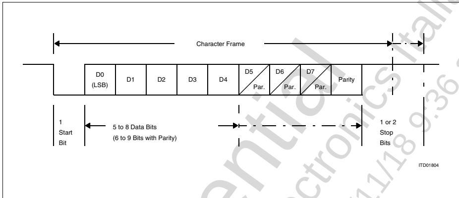
Figure 49 Asynchronous Character Frame
