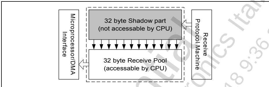
Figure 9 SCC Receive FIFO
