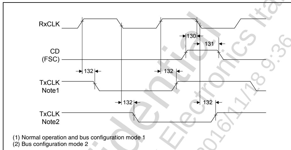
Figure 85 Clock Mode 5 Frame Synchronisation Timing
