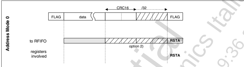
Figure 46 HDLC Receive Data Processing in Address Mode 0
