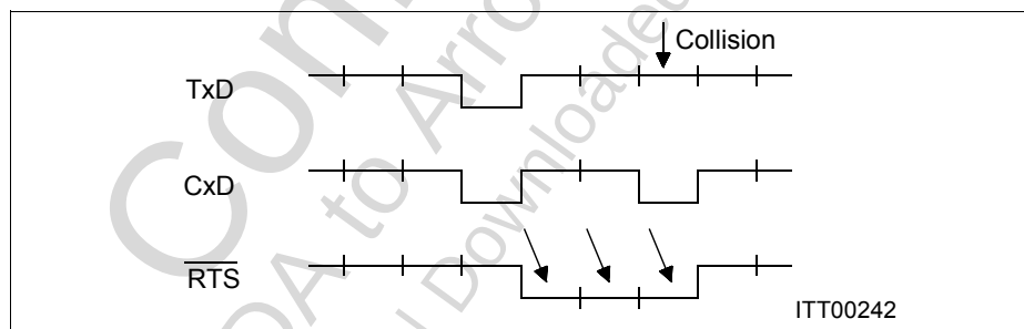
Figure 30 Request-to-Send in Bus Operation
