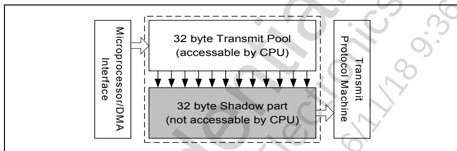
Figure 8 SCC Transmit FIFO
