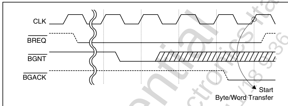
Figure 36 SEROCCO-D requests and gets the bus
