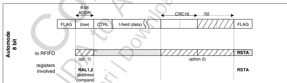
Figure 42 HDLC Receive Data Processing in 8 bit Automode
