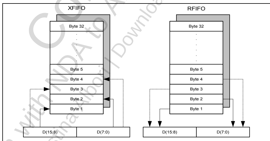
Figure 11 XFIFO/RFIFO Word Access (Motorola Mode)
