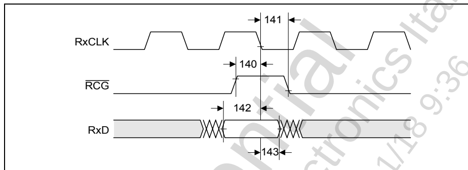
Figure 83 Clock Mode 4 Receive Gating Timing
