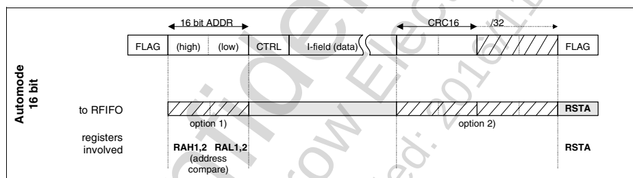
Figure 41 HDLC Receive Data Processing in 16 bit Automode
