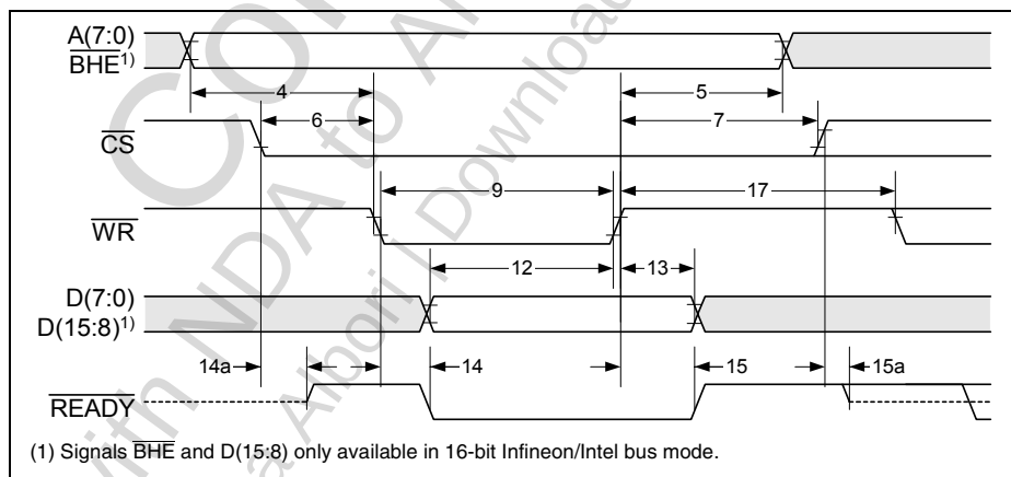
Figure 71 Infineon/Intel Write Cycle Timing (Slave Access)
