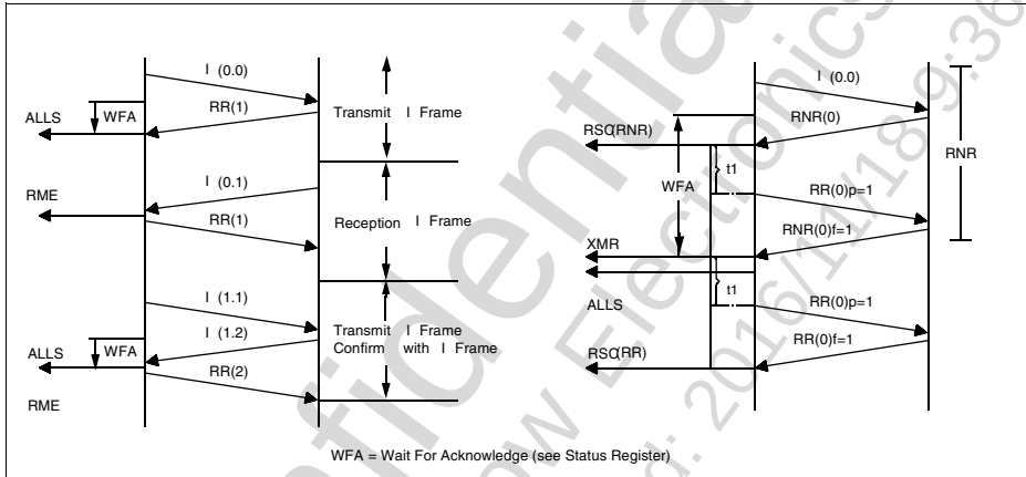
Figure 55 Transmission/Reception of I-Frames and Flow Control
