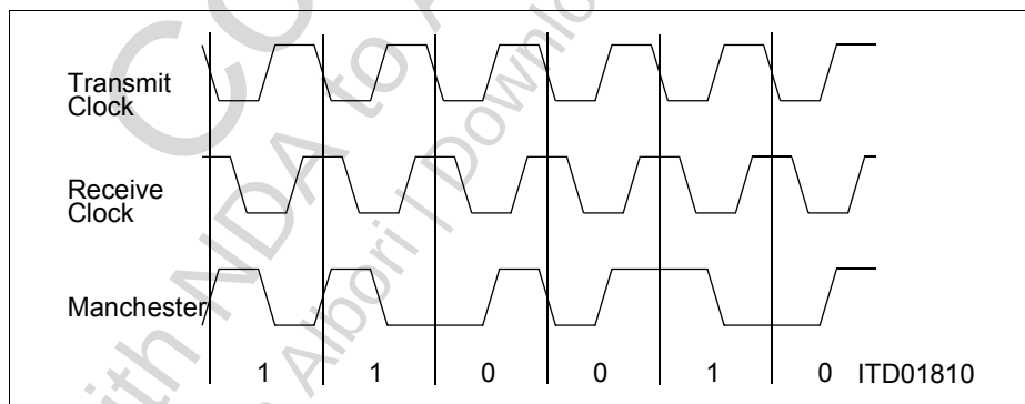
Figure 33 Manchester Data Encoding
