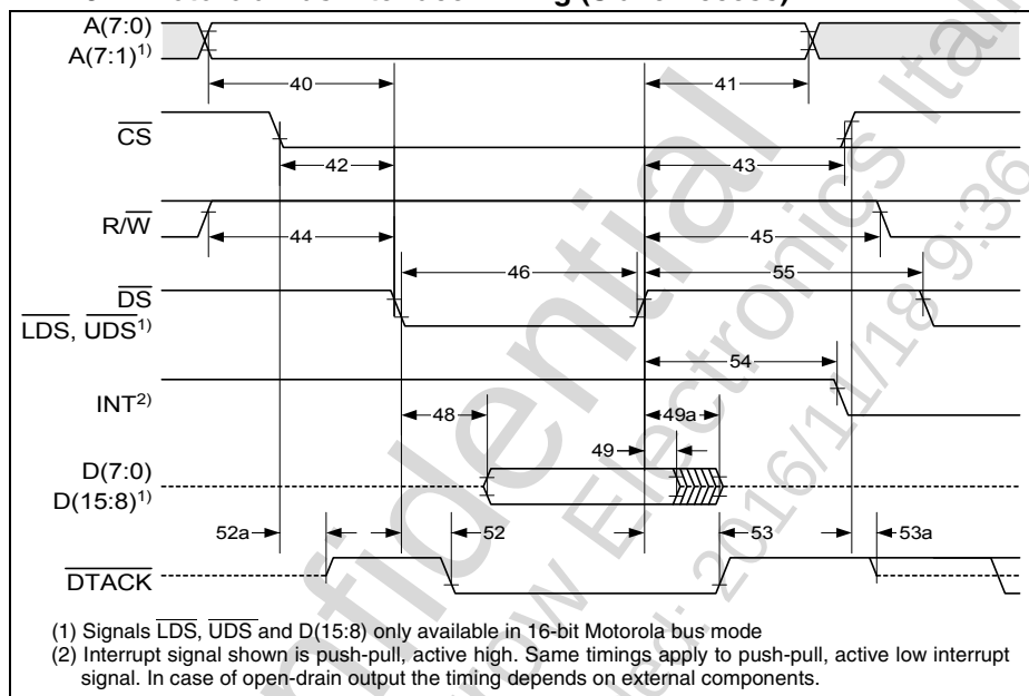
Figure 72 Motorola Read Cycle Timing (Slave Access)
