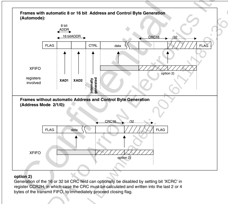
Figure 47 SCC Transmit Data Flow (HDLC Modes)
