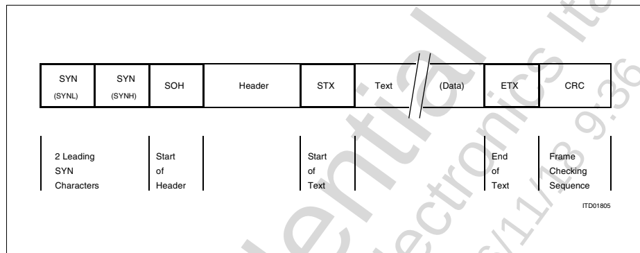
Figure 52 BISYNC Message Format
