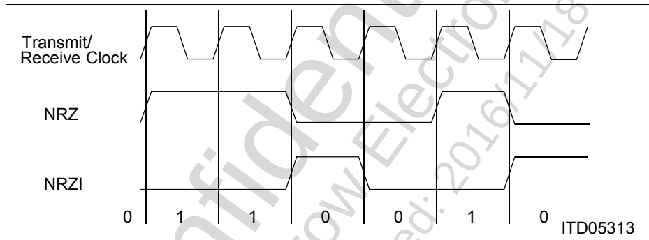
Figure 31 NRZ and NRZI Data Encoding
