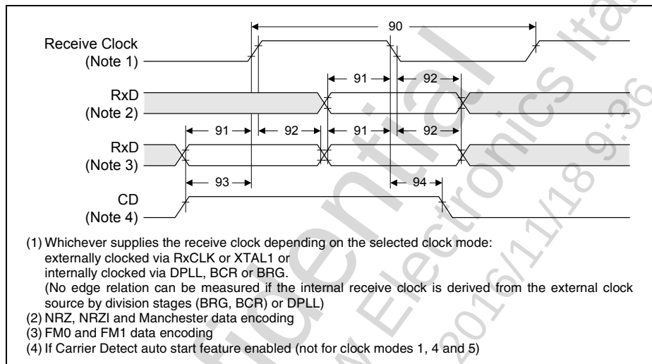
Figure 80 Receive Cycle Timing
