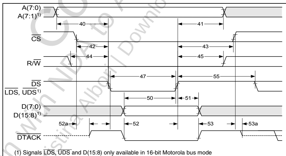
Figure 73 Motorola Write Cycle Timing (Slave Access)
