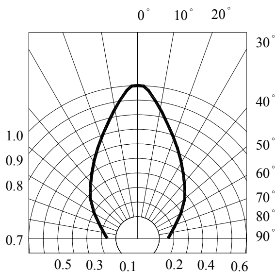
RADIATION DIAGRAM
