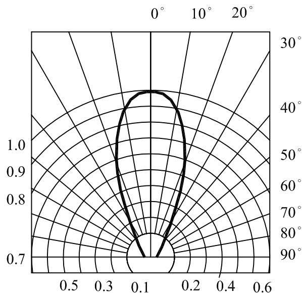
RADIATION DIAGRAM
