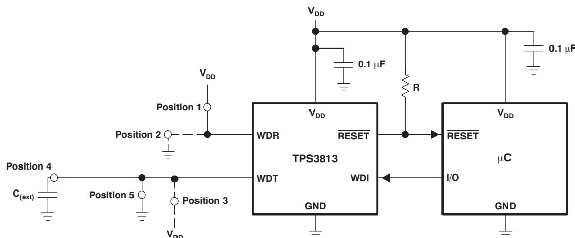
Figure 7. Application Example
