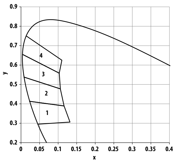
Avago Cyan Color Bin on CIE Chromaticity Diagram
