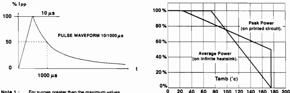
Figure 1: Power dissipation derating versus ambient temperature
